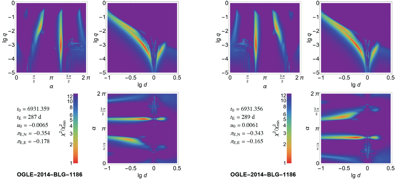
Figure 7. Exploration of binary-lens parameter space. Colour-coded values of \chi^2 for the peak data as a function of the binary-lens parameters ( d , q , \alpha ) as three diagrams of \chi^2 as a function of (\lg q, \alpha) , (\lg d, \lg q) , and (\lg d, \alpha) , where each reported value of \chi^2 corresponds to the minimum over the remaining third parameter. These diagrams have been positioned so that all three parameters corresponding to local minima can readily be identified. The parameters ( t_0 , t_E , u_0 , \pi_{E,N} , \pi_{E,E} ) have been kept fixed to values suggested by single-lens point-source parallax models for the off-peak data for u_0 < 0 or u_0 > 0 , respectively (c.f. Tables 3 and 4), and only the baseline fluxes F_{\text{base}}^{[j]} and the blend ratios g^{[j]} have been adjusted for each (d, q, \alpha) in order to minimize \chi^2 . The colour scale has been normalized, so that the absolute minimum corresponds to the red end, while a single lens or any configuration with a larger \chi^2 corresponds to the purple end. While for small mass ratios q , one finds an ambiguity d \leftrightarrow d^{-1} for the separation parameter, the valleys distinguished by the trajectory angle \alpha correspond to the three possible types for the specific morphology observed in the light curve, illustrated in Fig. 8.
